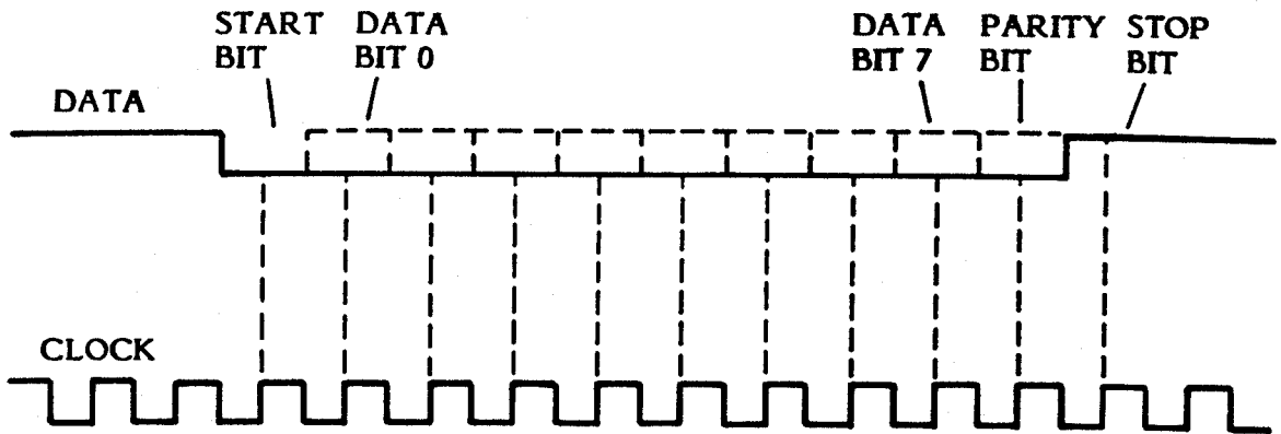
Figure 6-0 DATA FORMAT
