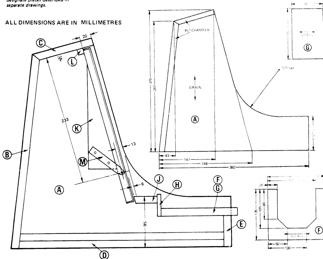
Fig.2. Cabinet assembly. Letters designate pieces described in separate drawings.
