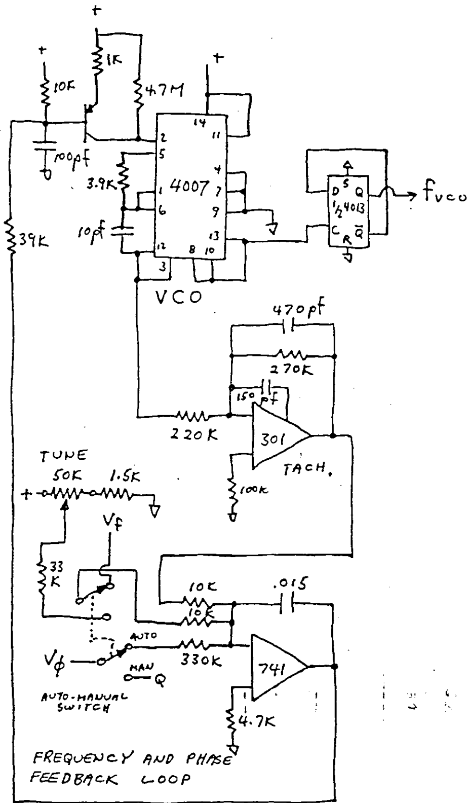
POLY-BOX VCO & SERVO LOOPS
